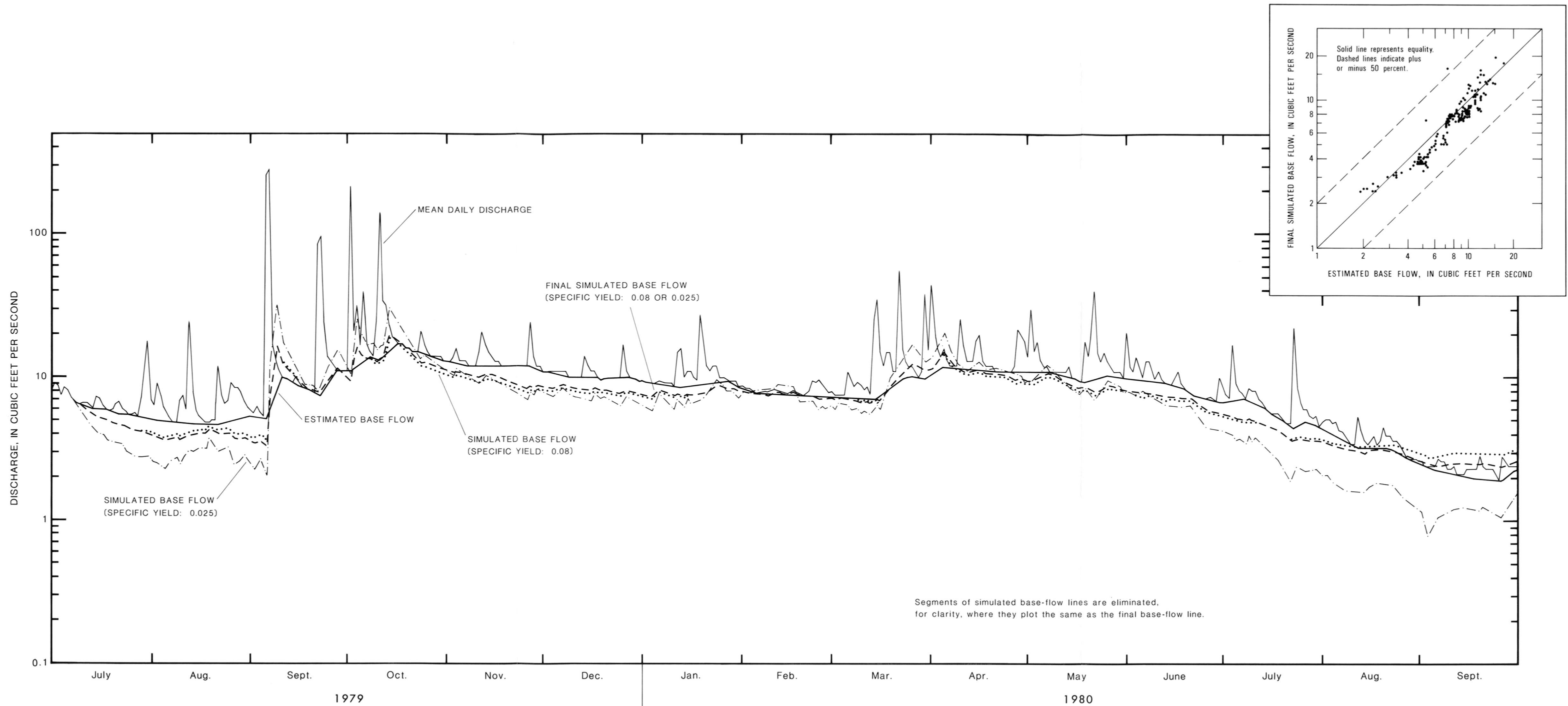
Figure 25. — Simulated base flows of Cattail Creek compared with estimated base flows at streamflow site 11, July 1979 to September 1980.
