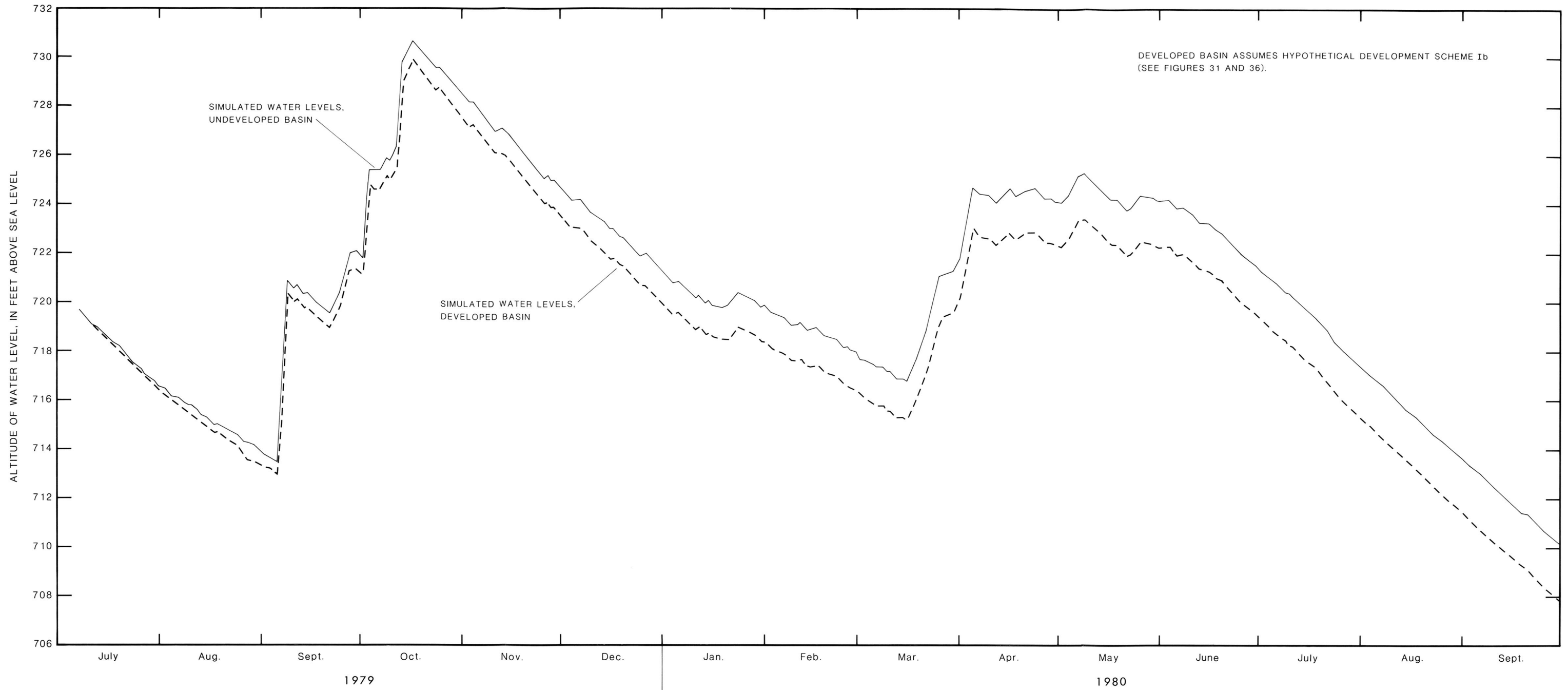
Figure 50. — Comparison of simulated water levels at cell B for developed (scheme 1b) and undeveloped basin, July 1979 to September 1980.
