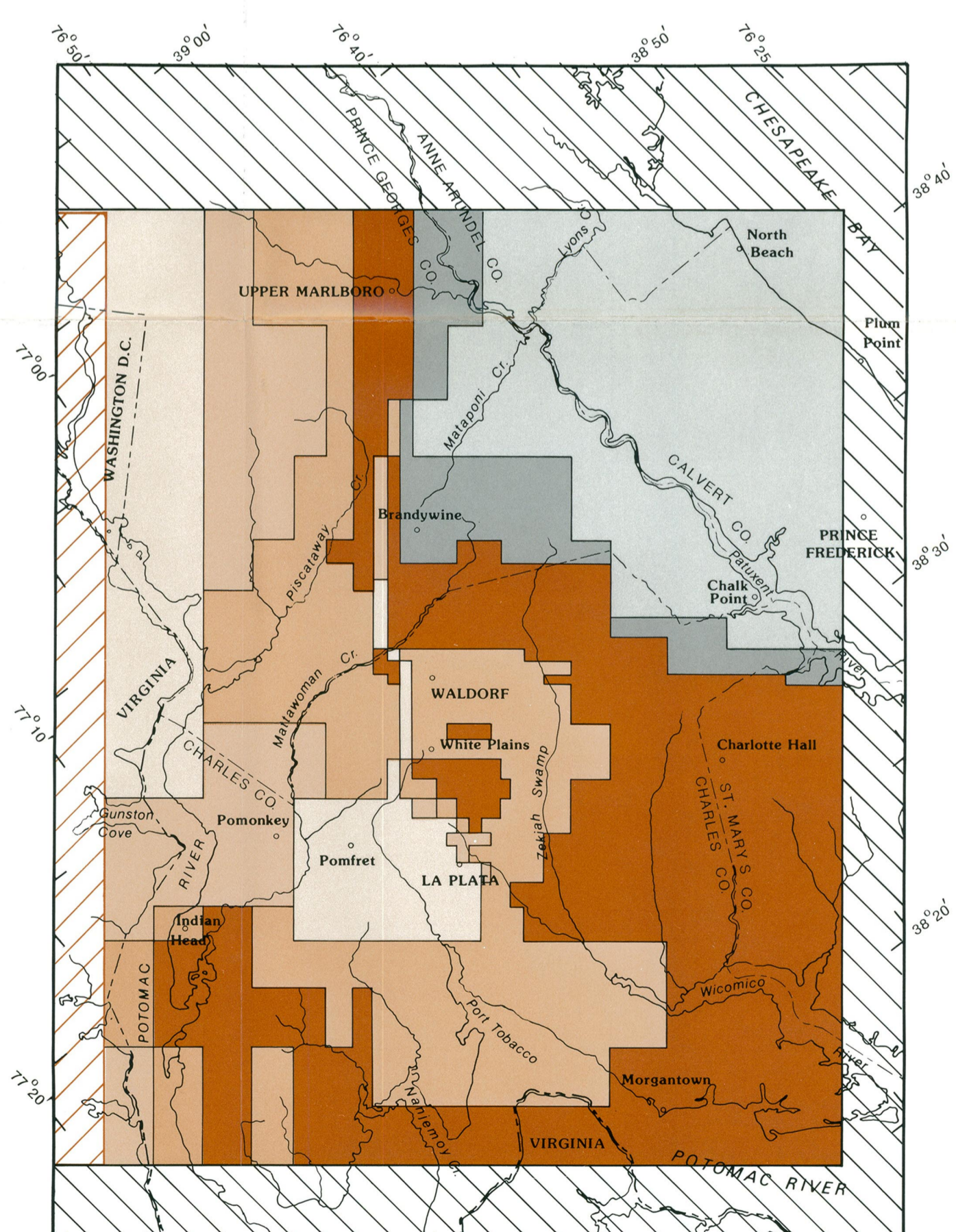
LA PLATA AQUIFER AND CORRELATIVE SANDS (G)
