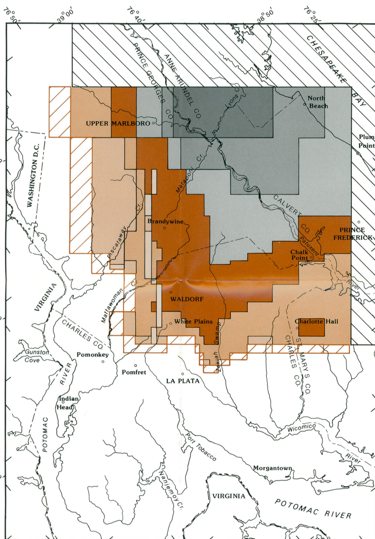
MAGOTHY AQUIFER (C)
