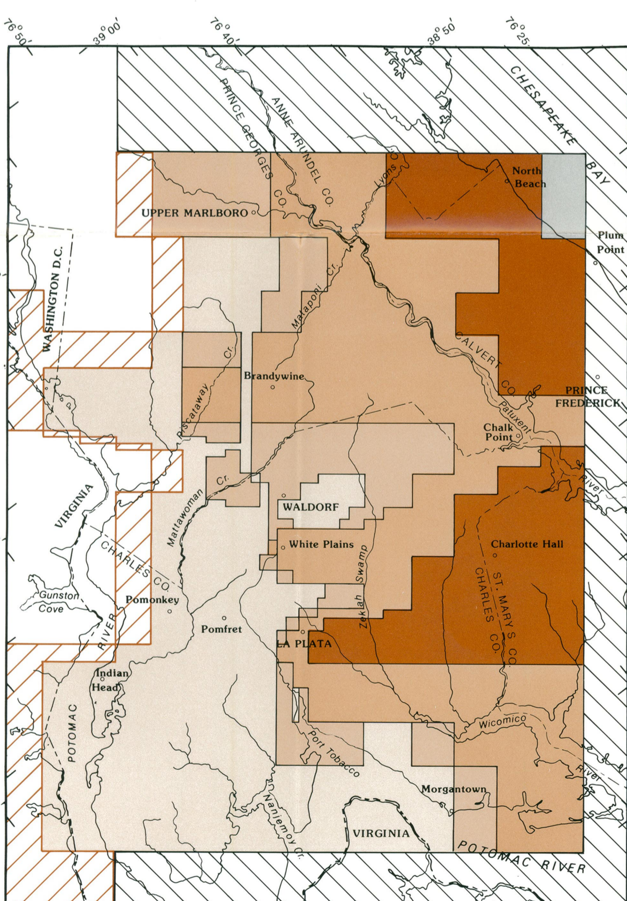
WHITE PLAINS AQUIFER AND CORRELATIVE SANDS (F)
