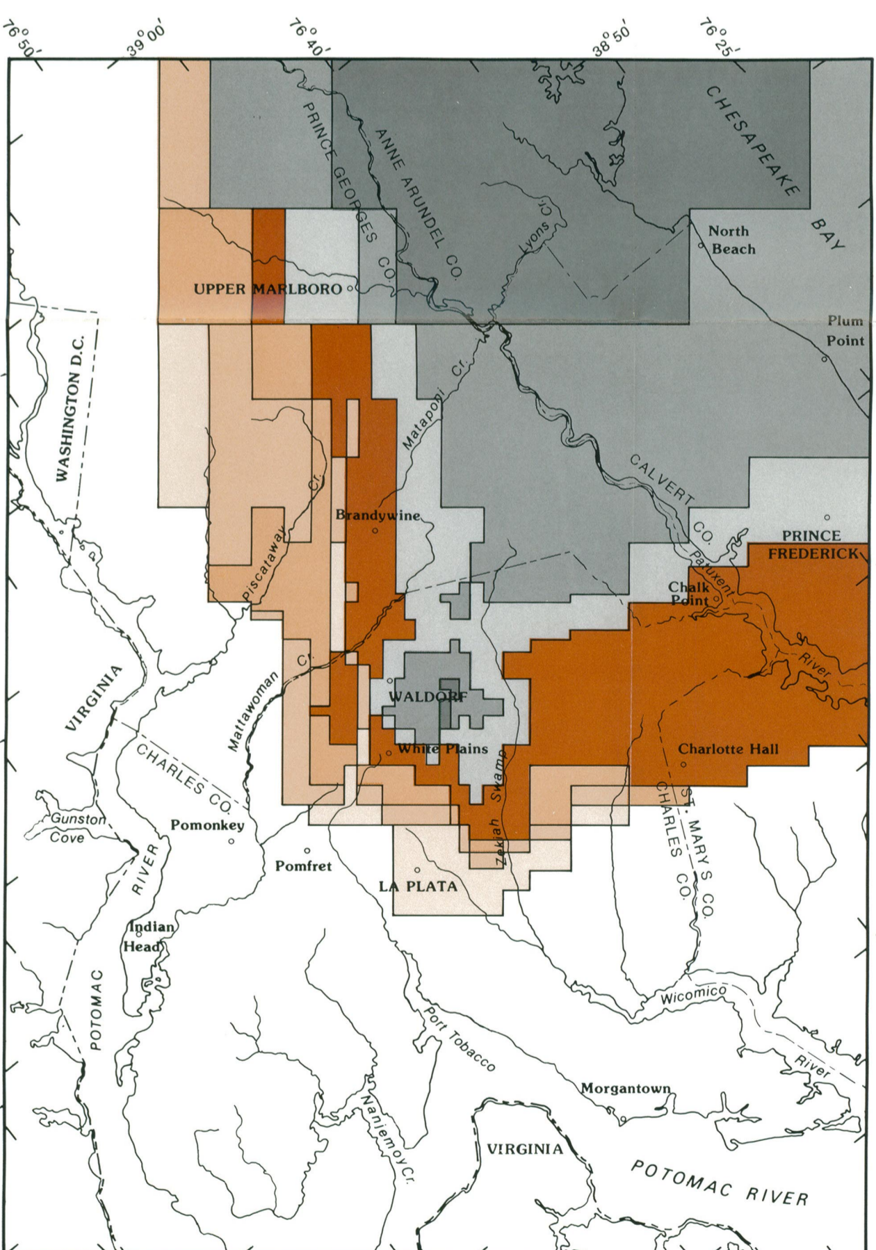
WALDORF AQUIFER SYSTEM AND CORRELATIVE SANDS (E)
