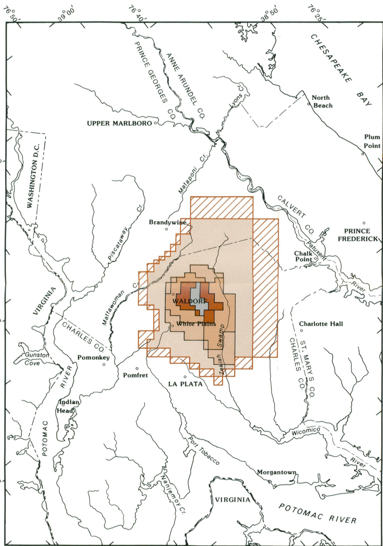
MONMOUTH AQUIFER (B)
